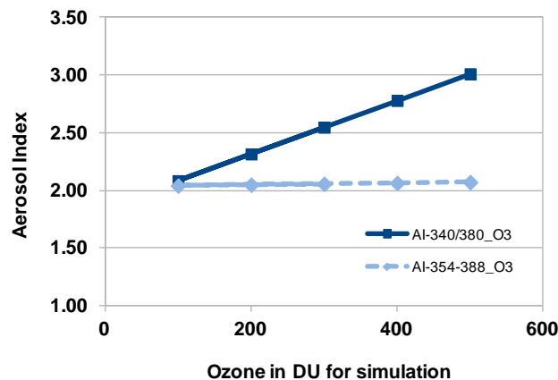
Figure 4-9. Bias in UVAI resulting from changing ozone concentration in simulation while fixing retrieval ozone concentration at 300 DU. AI_{340/380} is shown as dark blue, solid line and AI_{354/388} in light blue with dashed line.
